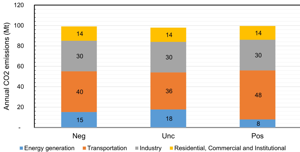
Figure 6: Annual sectorial CO2 emissions for 2030 (Mt).
