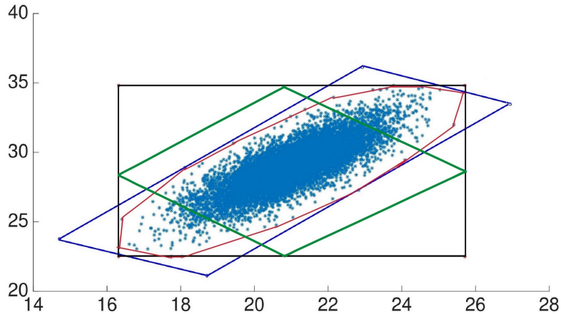
Figure 2: Definition of uncertainty sets for two correlated uncertain parameters. Black: Box [33]; Green: Budget [34]; Red: Convex hull; Blue: PCA-based uncertainty set including correlation [35]. Source:[35]
